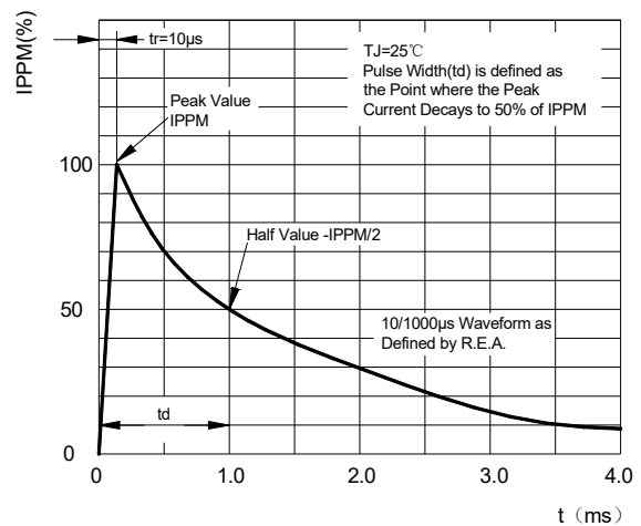
FIG2: Pulse Waveform
